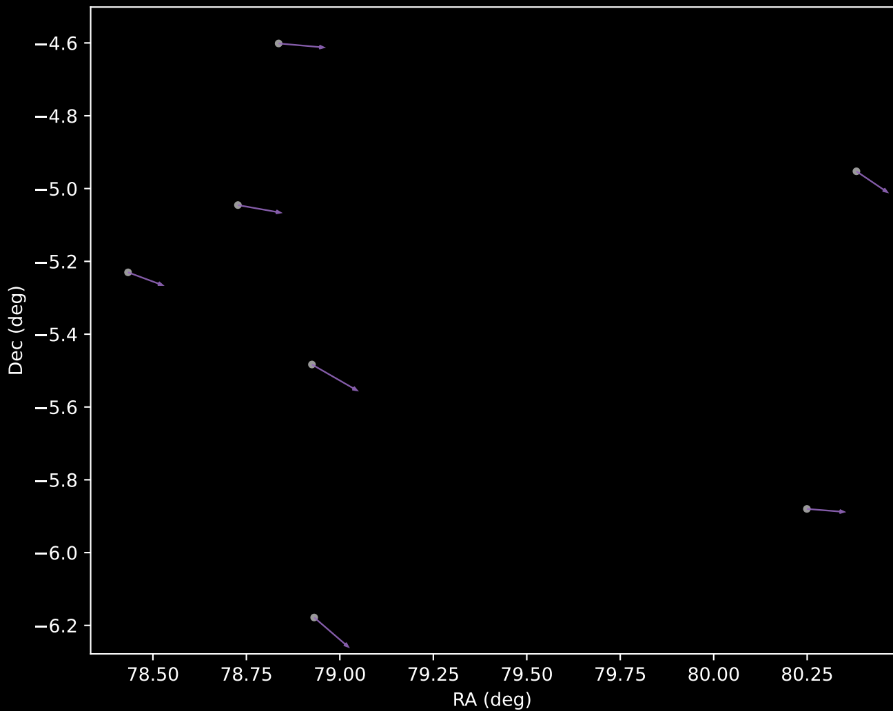
APOGEE DR17 Cluster 8 Proper Motion Vectors (n=7)
