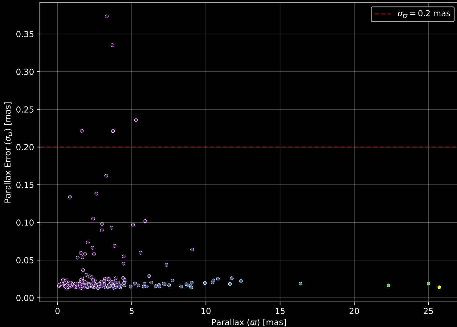
APOGEE DR17 Field: [K2_C3_061-52_btx] Parallax Quality (n= 211)
