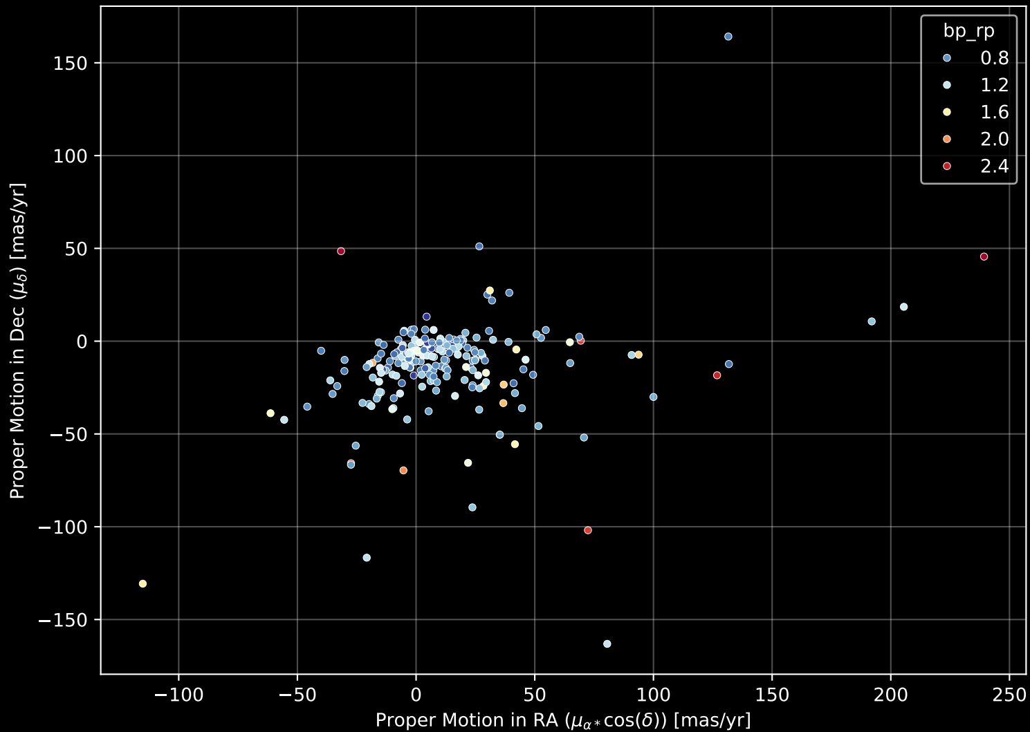
APOGEE DR17 Field: [K2_C3_061-52_btx] Proper Motion Diagram (n= 211)
