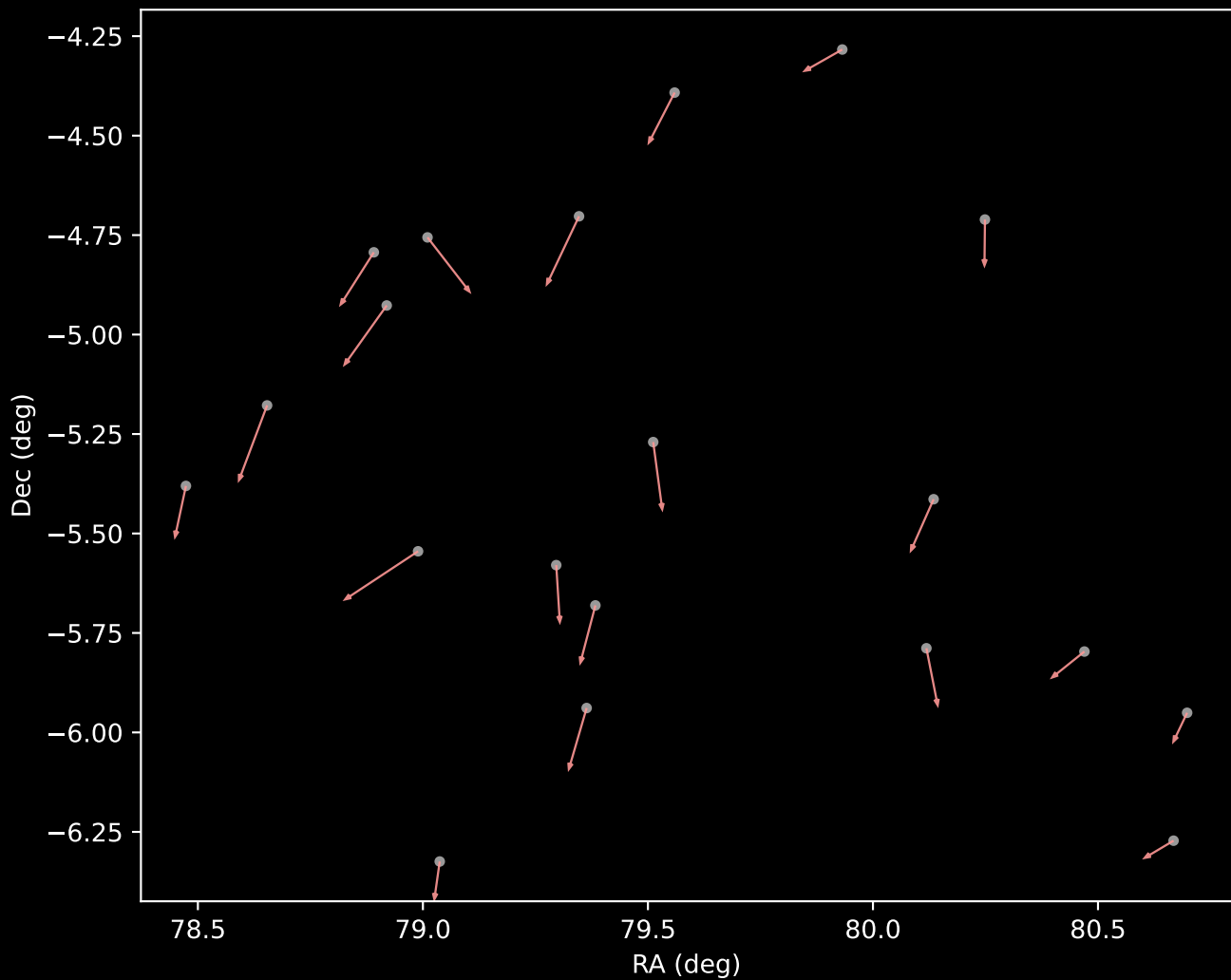
APOGEE DR17 Cluster 7 Proper Motion Vectors (n=20)
