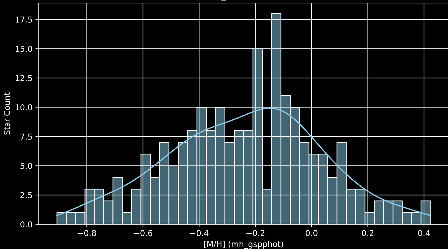
APOGEE DR17 Field: [K2_C3_061-52_btx [M/H] (mh_gspphot) (n= 211)
