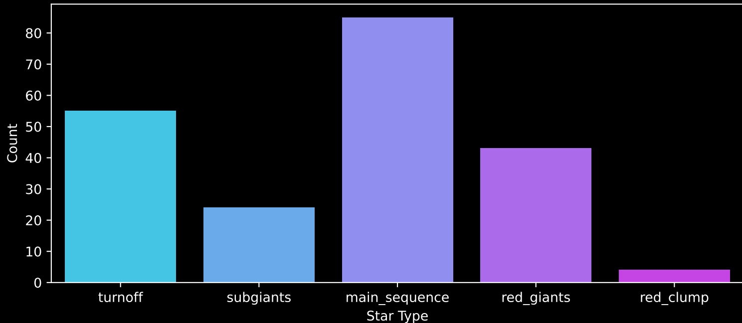
APOGEE DR17 Field: [K2_C3_061-52_btx] Count plot of Star Type
