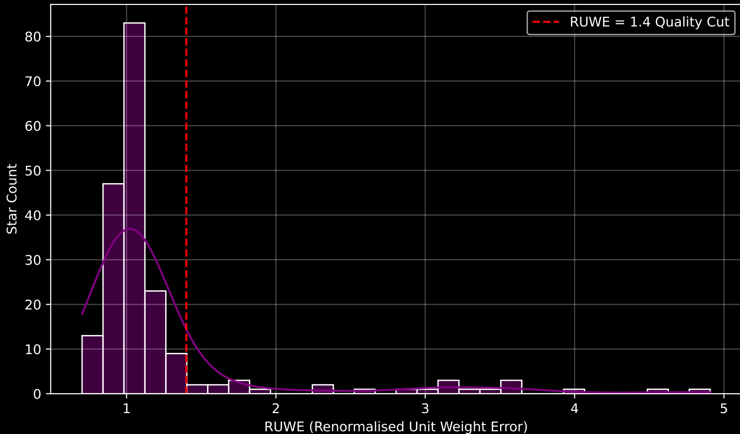
GAPOGEE DR17 Field [K2_C3_061-52_btx] RUWE Distribution (n= 199)
