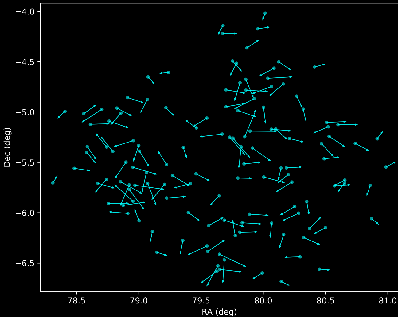
APOGEE DR17 Noise Stream Proper Motion Vectors (n=129)
