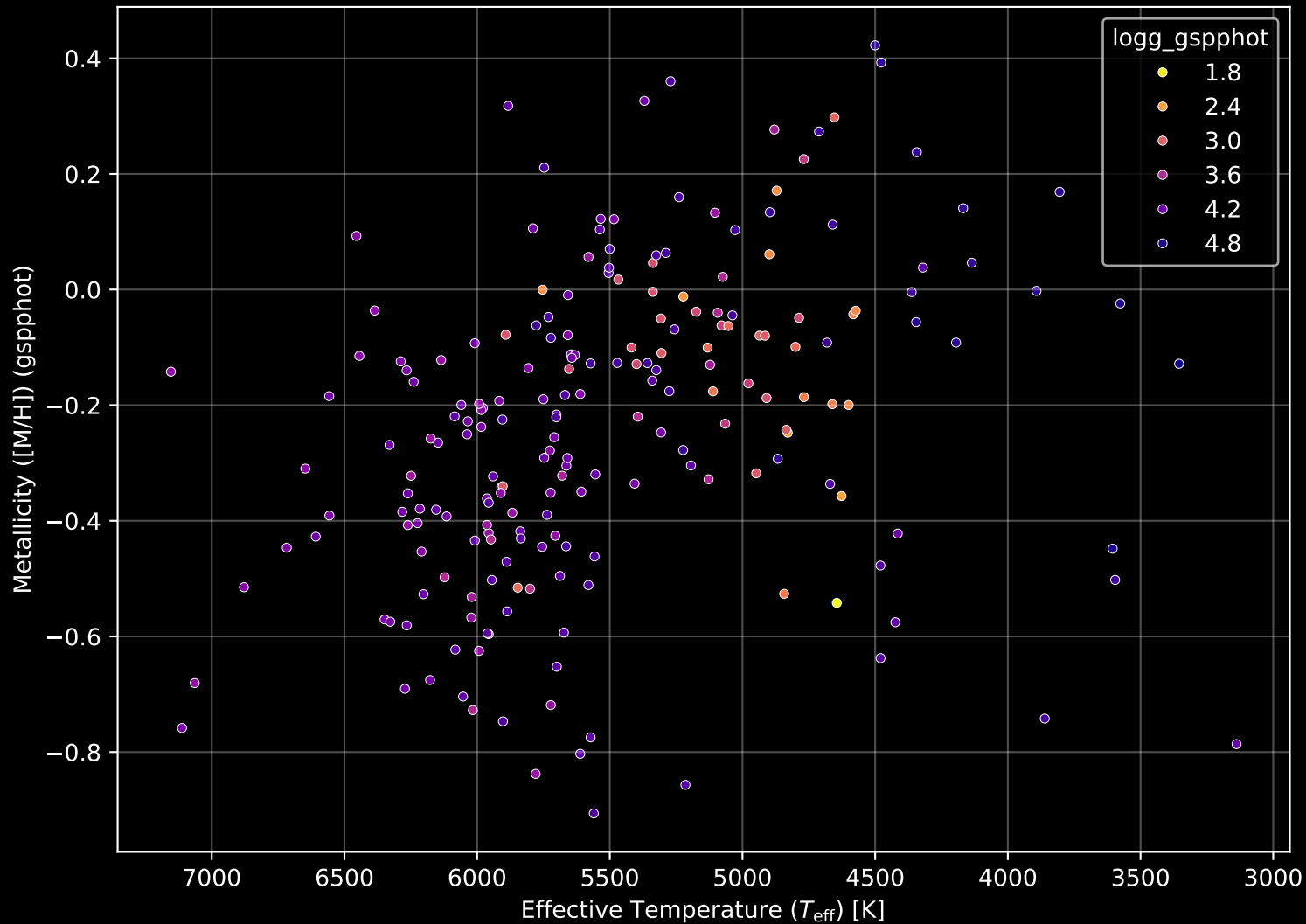
APOGEE DR17 Field: [K2_C3_061-52_btx] Stellar Population Parameters (n= 211)
