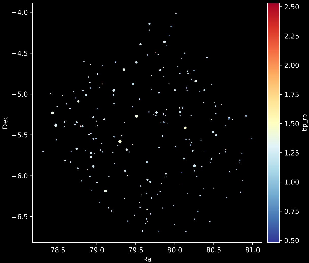
APOGEE DR17 Field: [K2_C3_061-52_btx] Stars: 211
